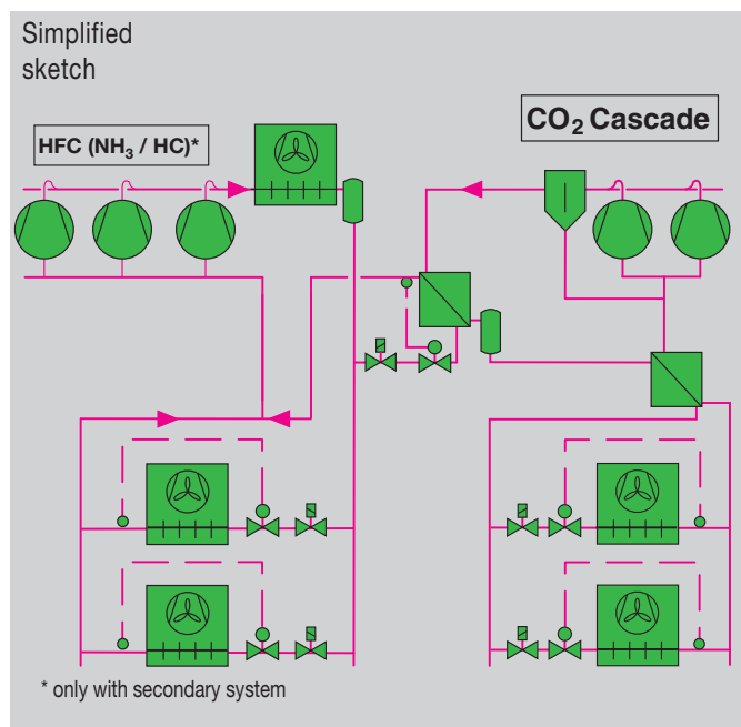
Fig. 30/2 Conventional refrigeration system combined with CO 2 low temperature cascade
