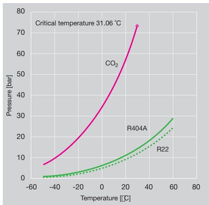
Fig. 29/2 R744(CO 2 )/R22/R404A – comparison of pressure levels
