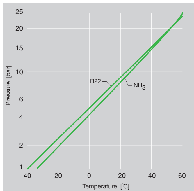
Fig. 26 NH 3 /R22 – comparison of pressure levels
